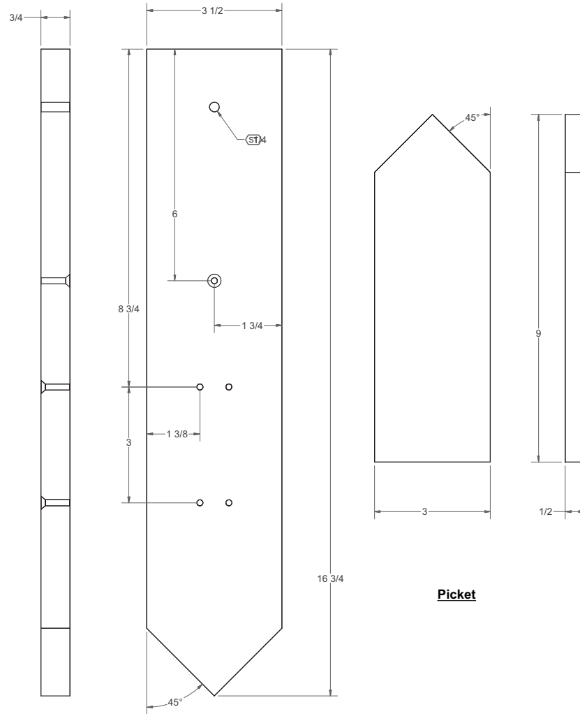
Mounting Board
