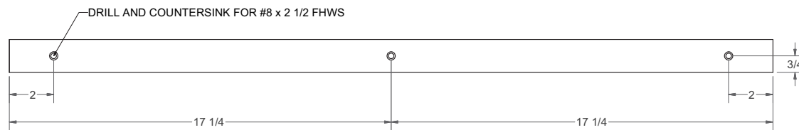
BASE SLAT CLEAT
