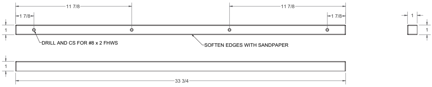
GATE GUIDE RAIL (NEED 4)
