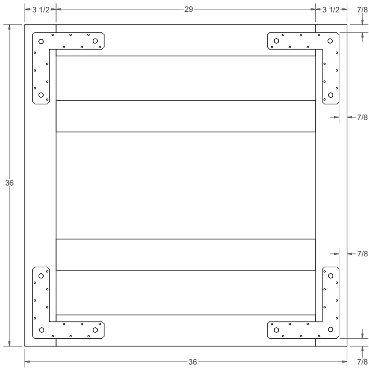
SIDE FRAME ASSEMBLY
